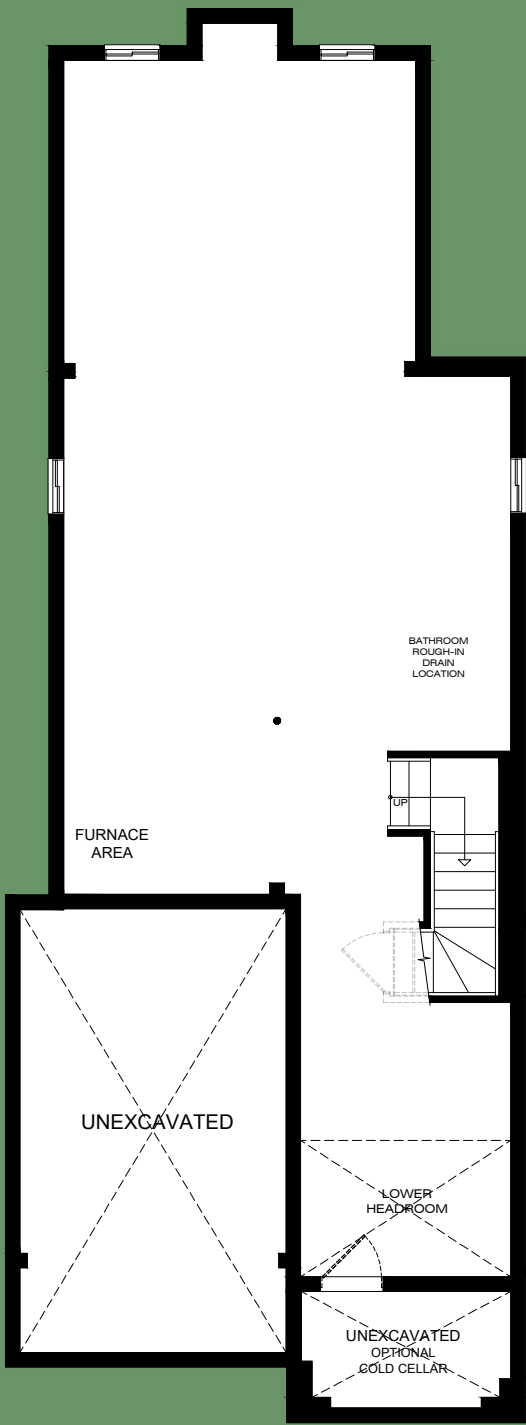
BASEMENT PLAN ELEVATION 'A' UNFINISHED BASEMENT
