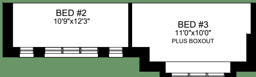
SECOND FLOOR PLAN ELEVATION 'B'
