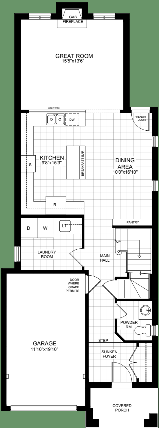
MAIN FLOOR PLAN ELEVATION 'A' (WITH MAIN FL LAUNDRY)
