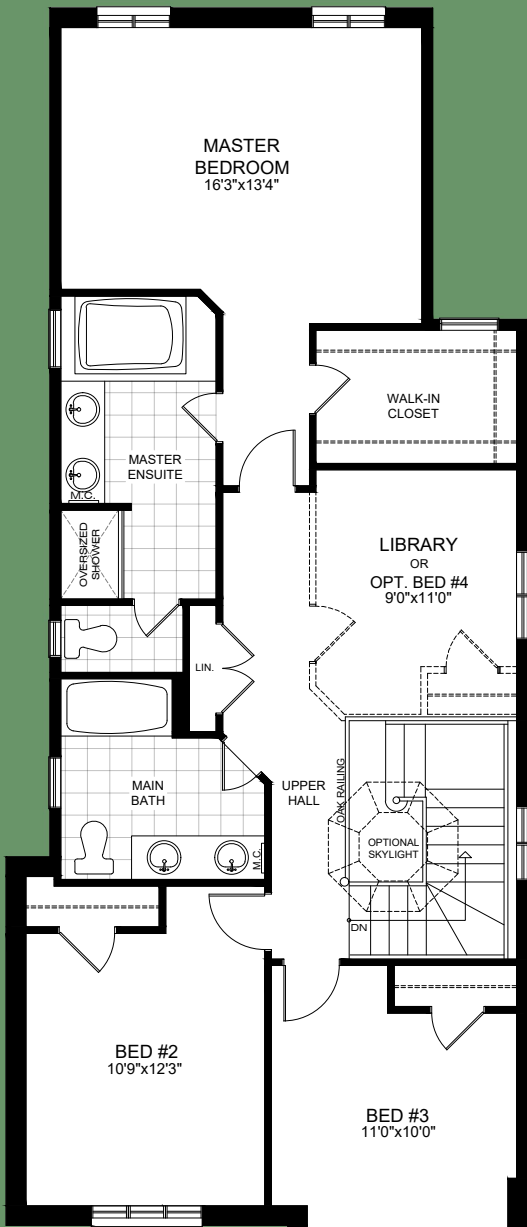
SECOND FLOOR PLAN ELEVATION 'A' (4 BED/LIBRARY - MAIN FL LAUNDRY)
