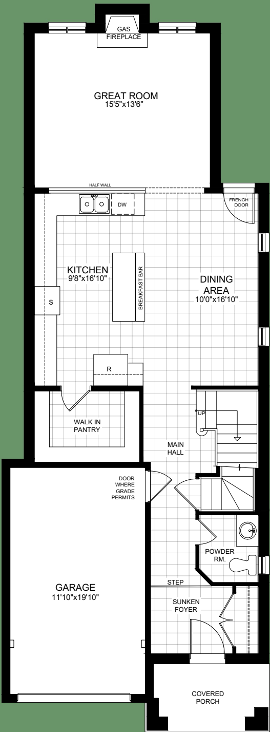
MAIN FLOOR PLAN ELEVATION 'A' (WITH SECOND FL LAUNDRY)
