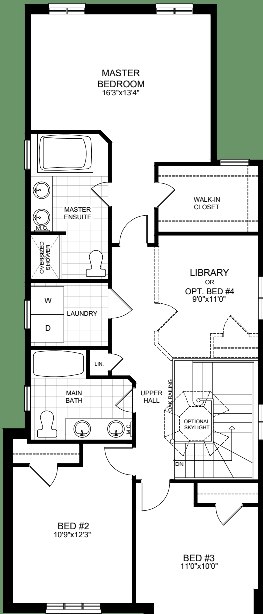
SECOND FLOOR PLAN ELEVATION 'A' (4 BED/LIBRARY - SECOND FL LAUNDRY)
