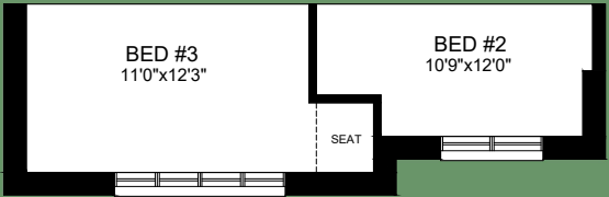
SECOND FLOOR PLAN ELEVATION 'C' (3 BEDROOM)
