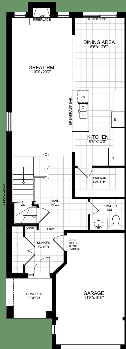
MAIN FLOOR PLAN ELEVATION 'B'
