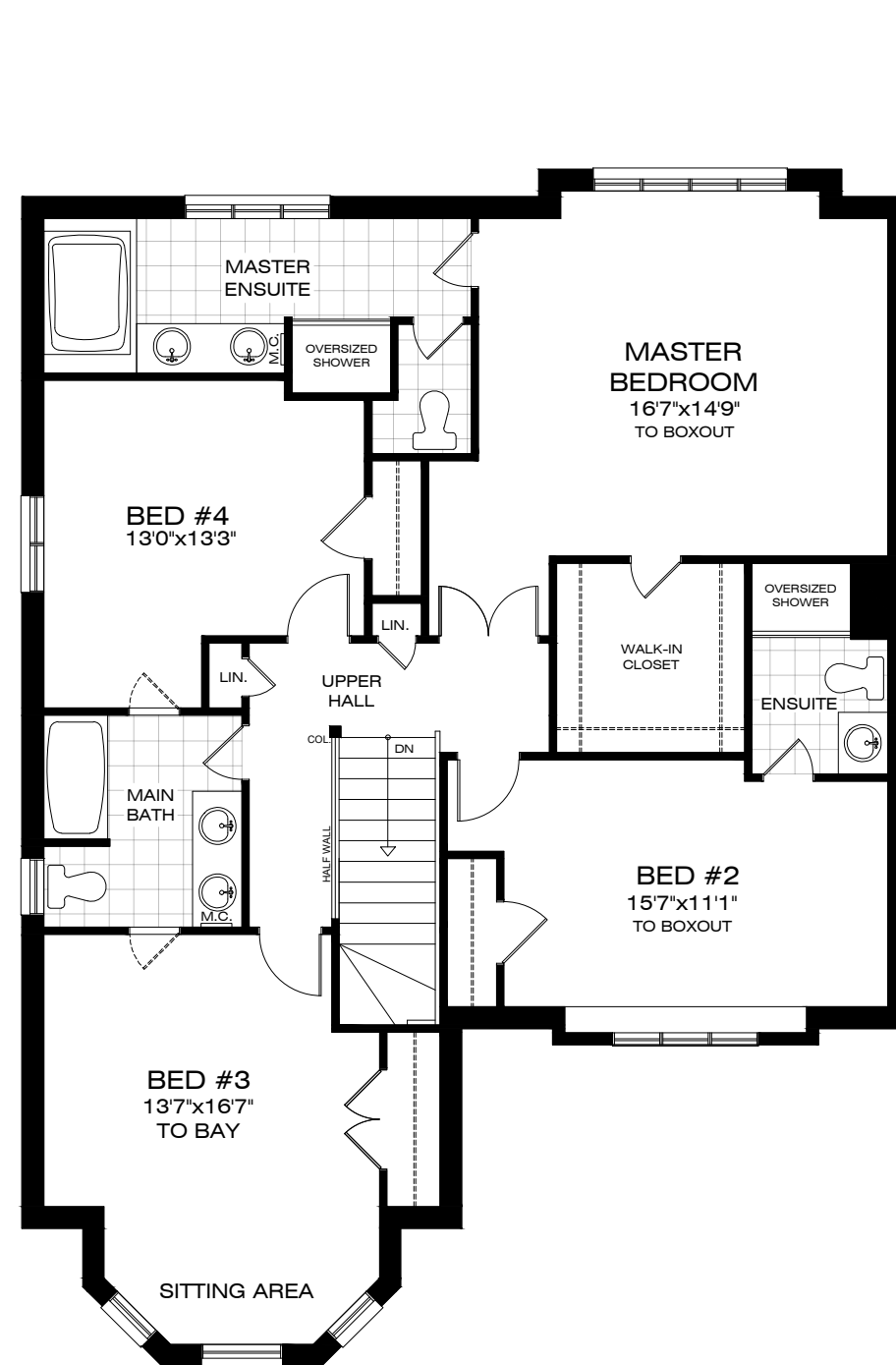
SECOND FLOOR PLAN ELEVATION A
