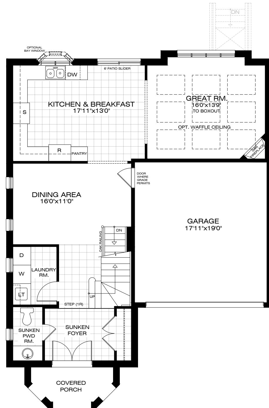
MAIN FLOOR PLAN ELEVATION A
