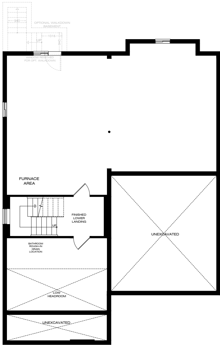
BASEMENT PLAN ELEVATION A
