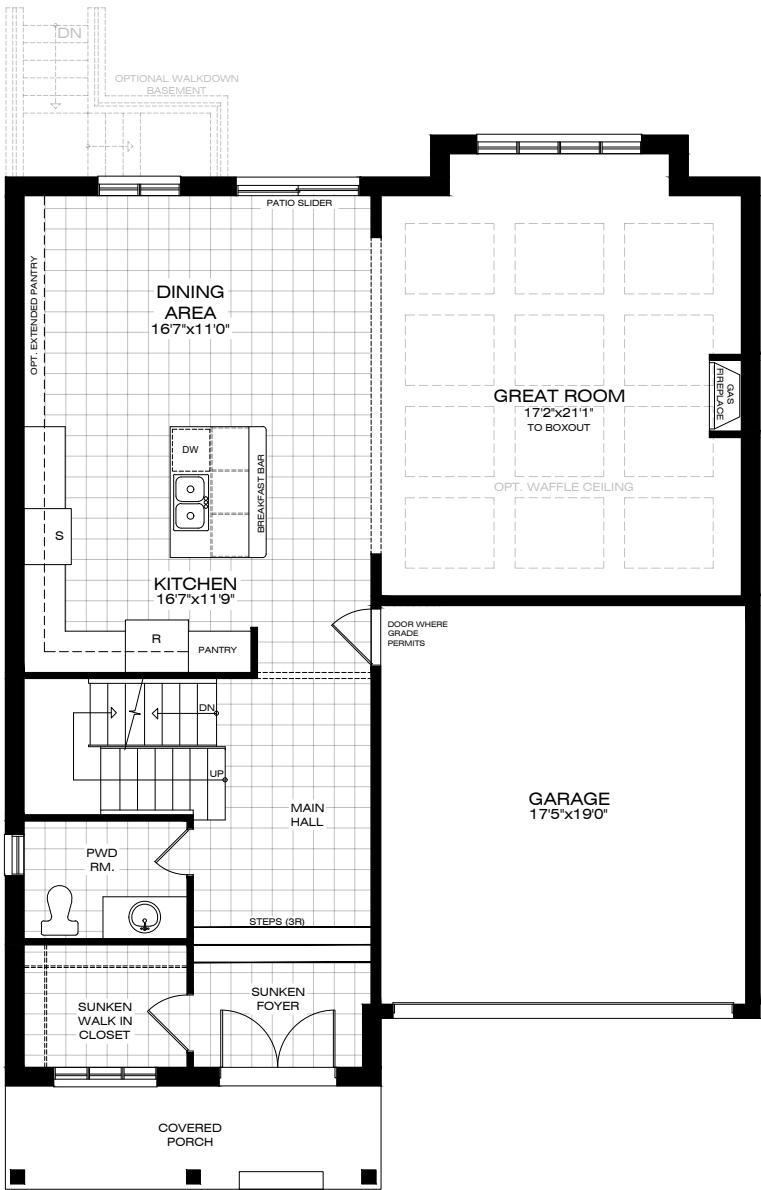
MAIN FLOOR PLAN ELEVATION A
