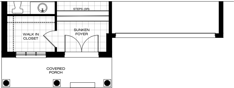
MAIN FLOOR PLAN ELEVATION B
