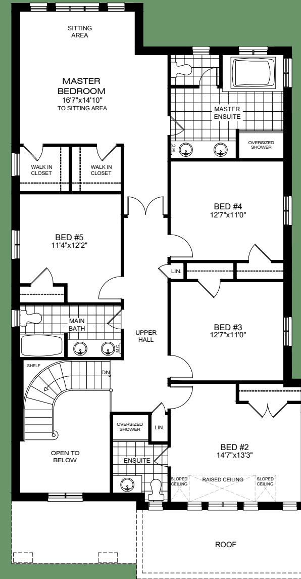
ALT. SECOND FLOOR PLAN ELEVATION A,B - 5 BEDROOM
