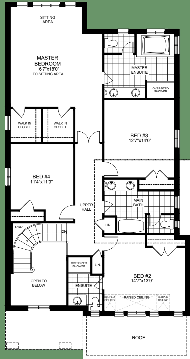
STD. SECOND FLOOR PLAN ELEVATION A,B - 4 BEDROOM
