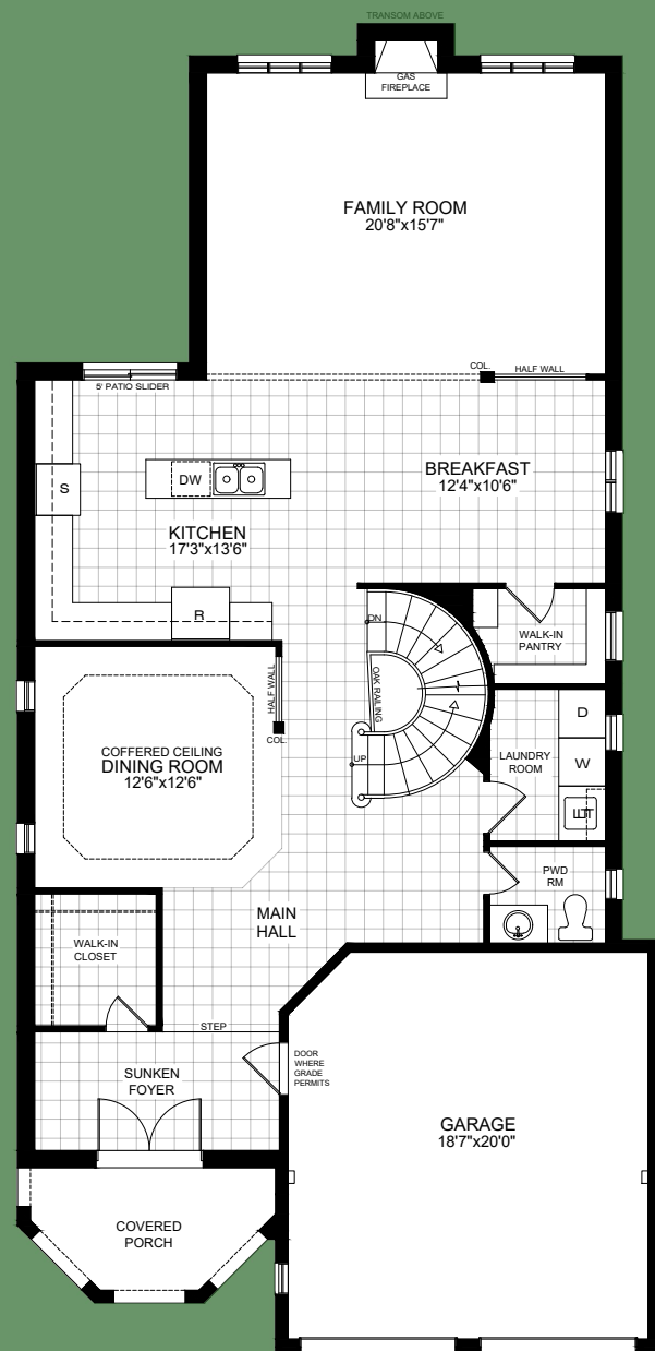
MAIN FLOOR PLAN ELEVATION B
