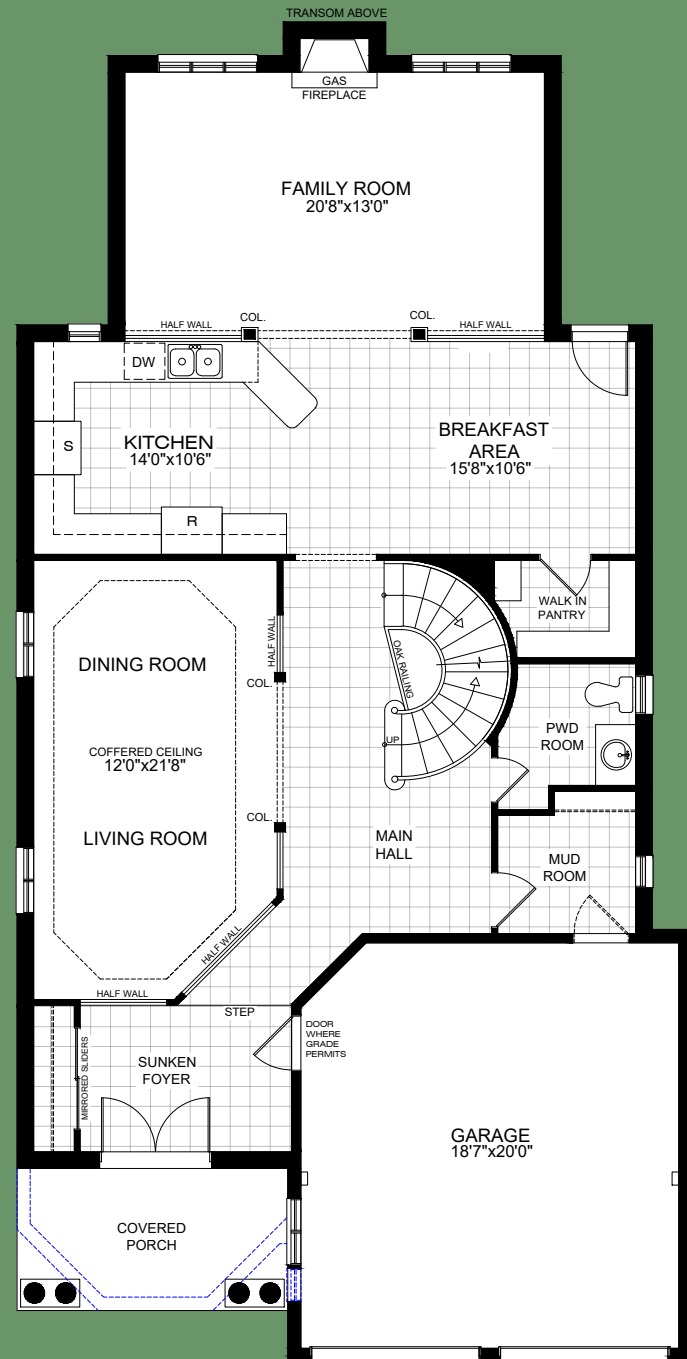
MAIN FLOOR PLAN ELEVATION A / ELEVATION B
