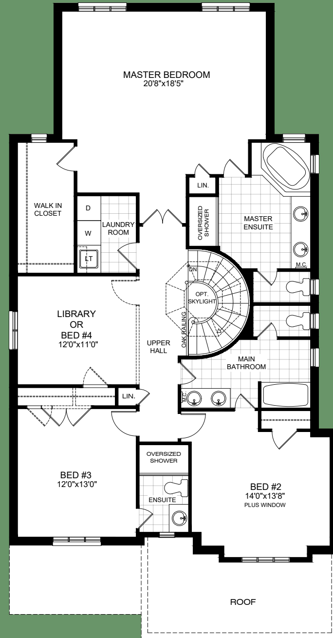
SECOND FLOOR PLAN ELEVATION A
