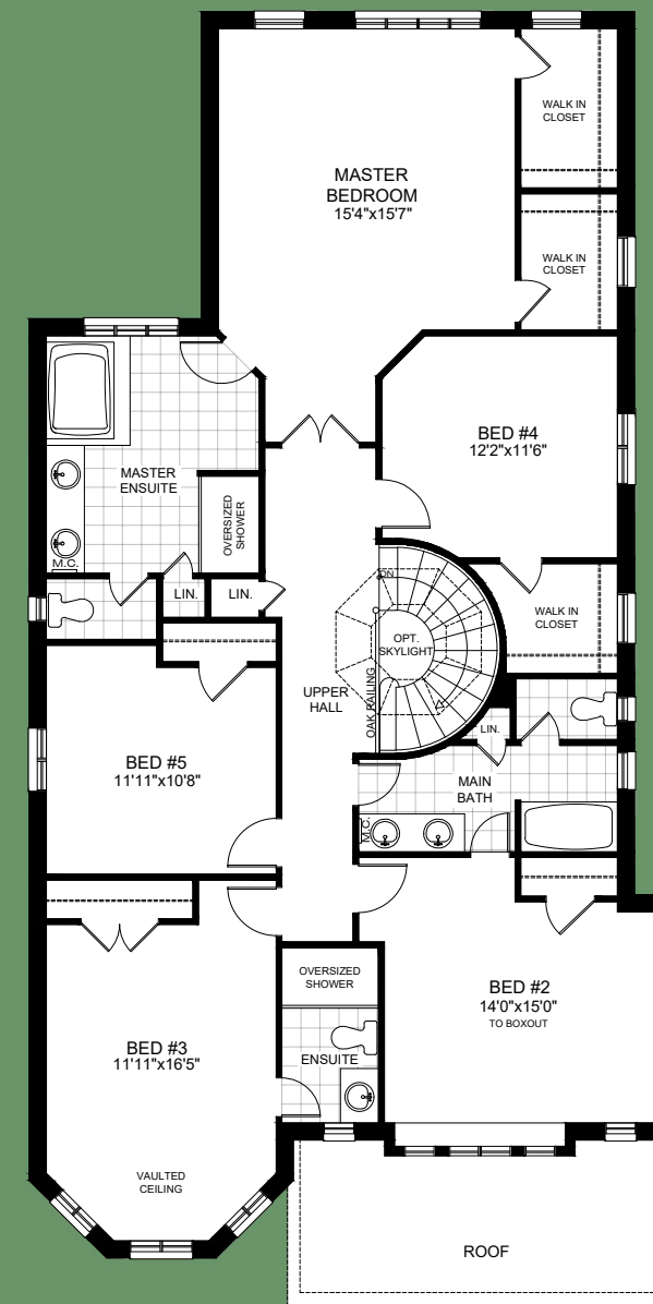
ALT. SECOND FLOOR PLAN ELEVATION B - 5 BEDROOM
