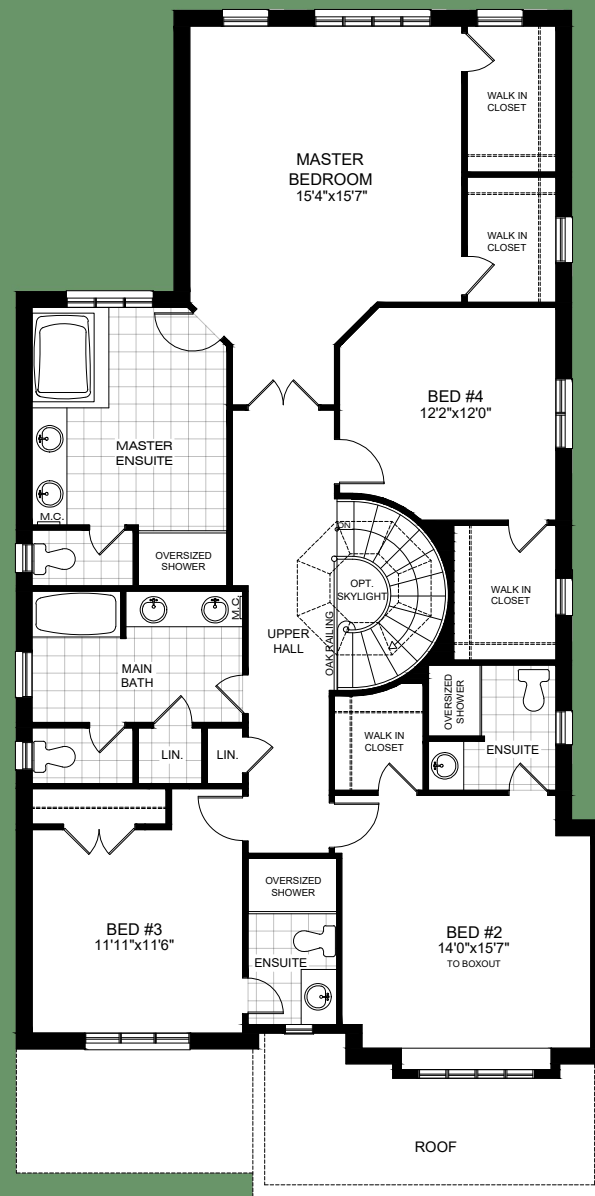
ALT. SECOND FLOOR PLAN ELEVATION A - 4 BEDROOM
