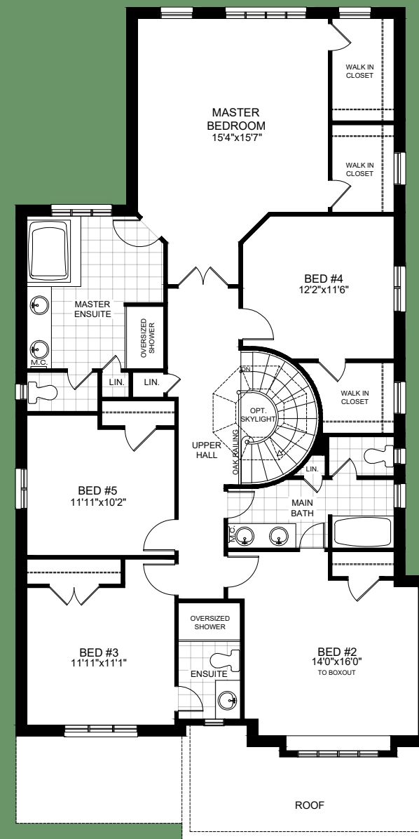
ALT. SECOND FLOOR PLAN ELEVATION A - 5 BEDROOM
