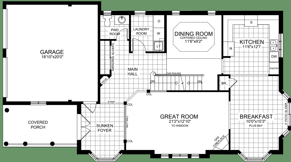
MAIN FLOOR PLAN ELEVATION A
