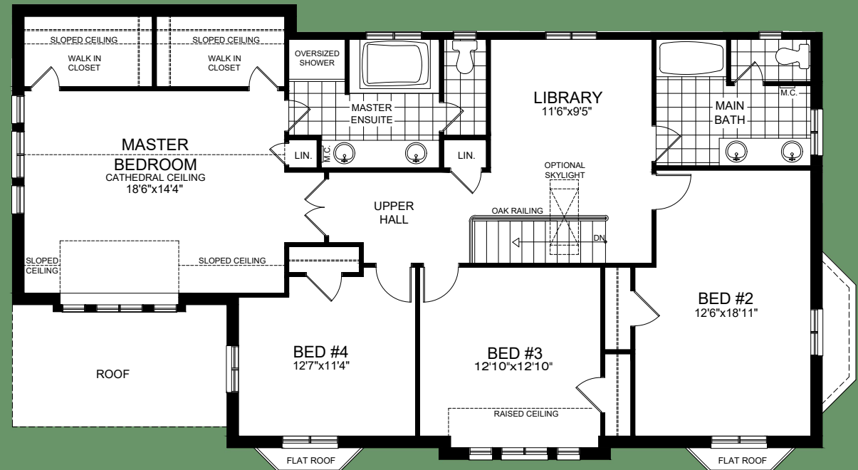
SECOND FLOOR PLAN WITH LIBRARY
