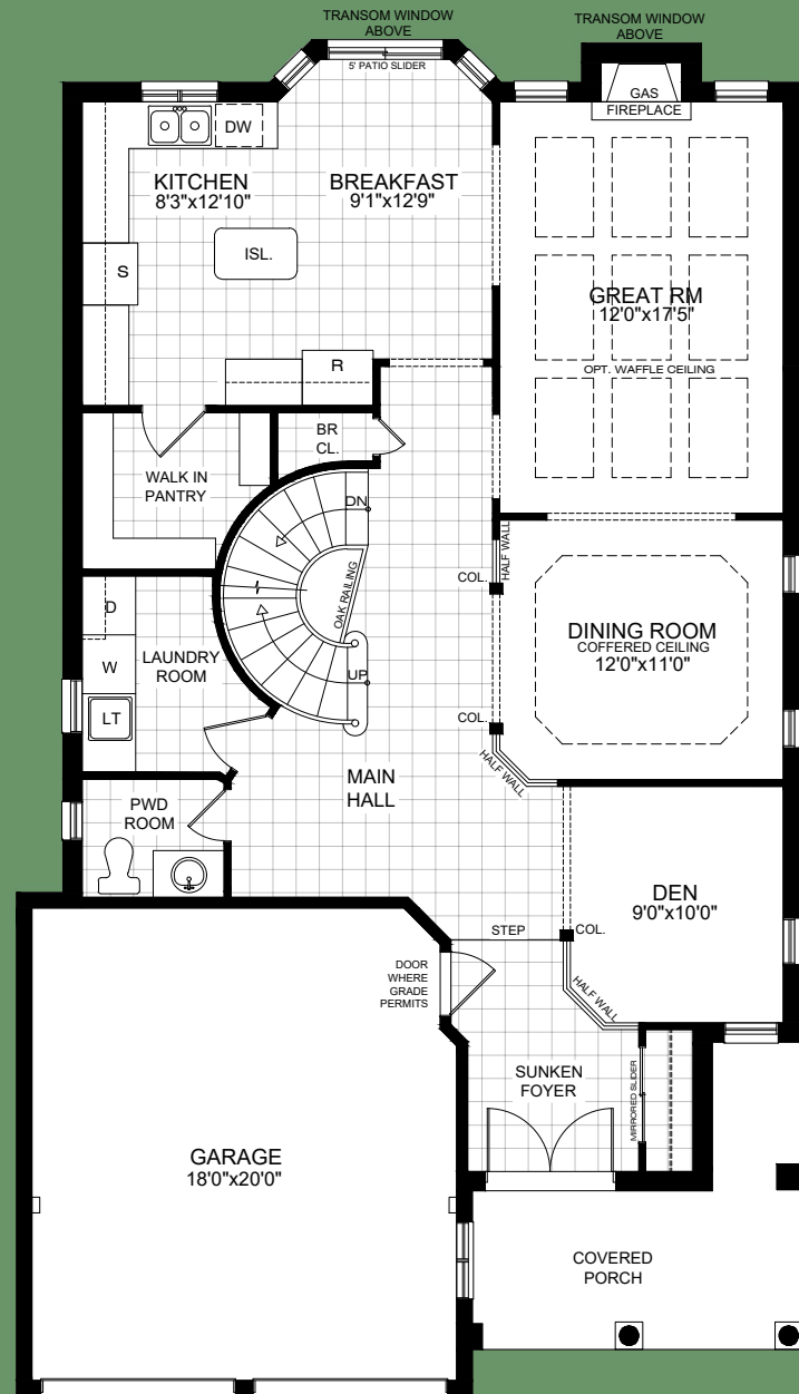
STD. MAIN FLOOR PLAN WITH DEN ELEVATION A,B
