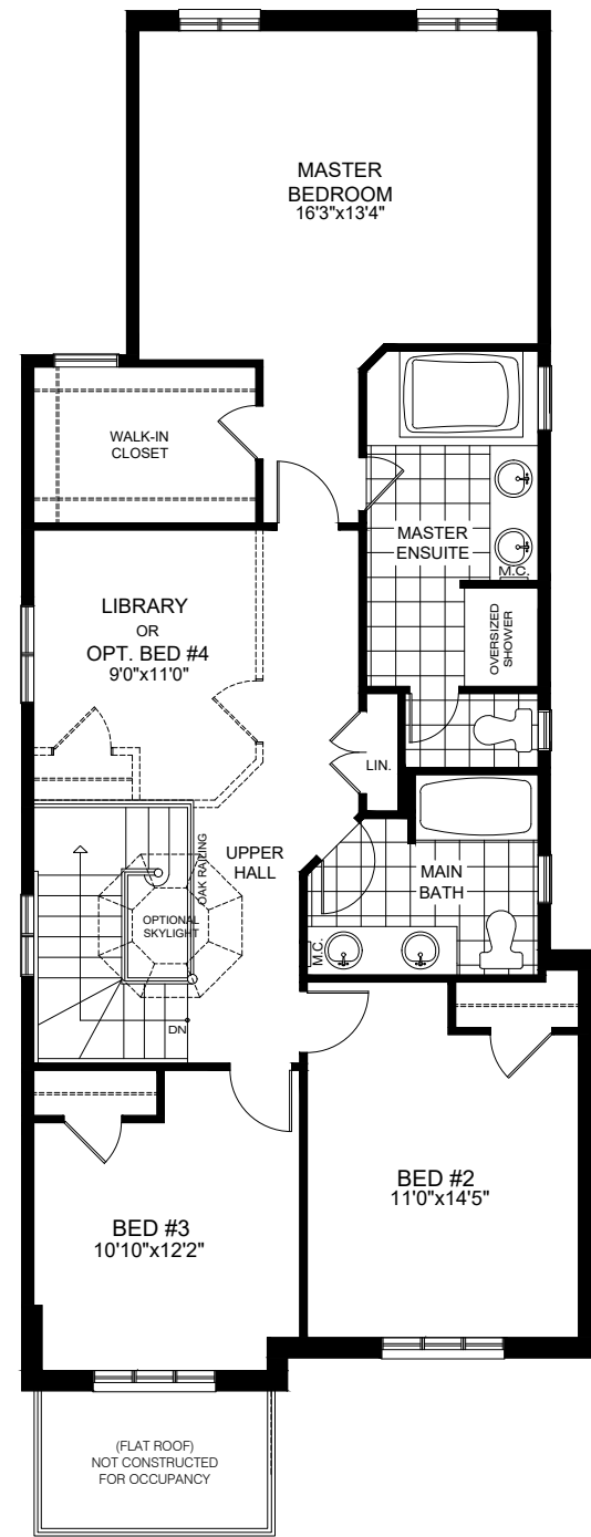
SECOND FLOOR PLAN ELEVATION 'A' (3 BEDROOM)
