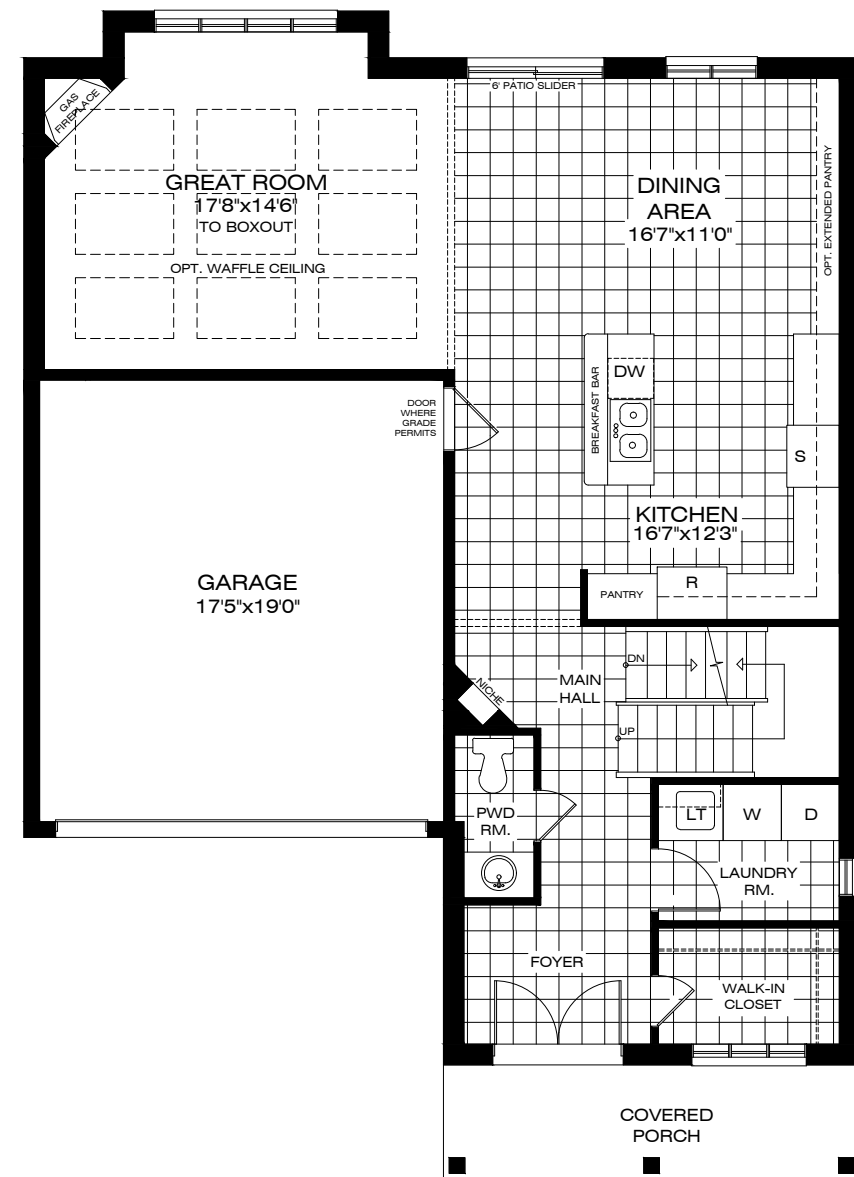
MAIN FLOOR PLAN ELEVATION A
