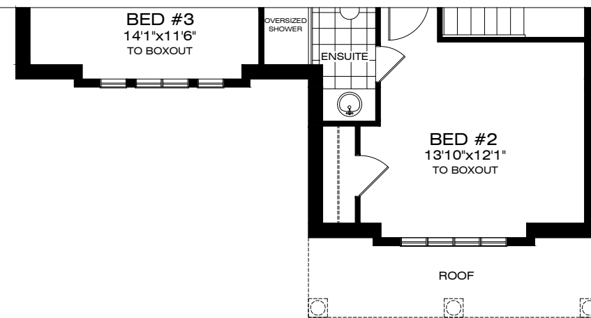
SECOND FLOOR PLAN ELEVATION B
