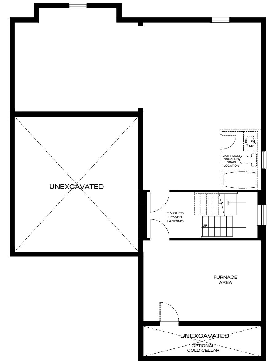
SECOND FLOOR PLAN ELEVATION A,B
