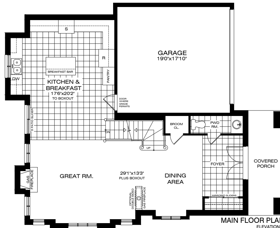
MAIN FLOOR PLAN ELEVATION A
