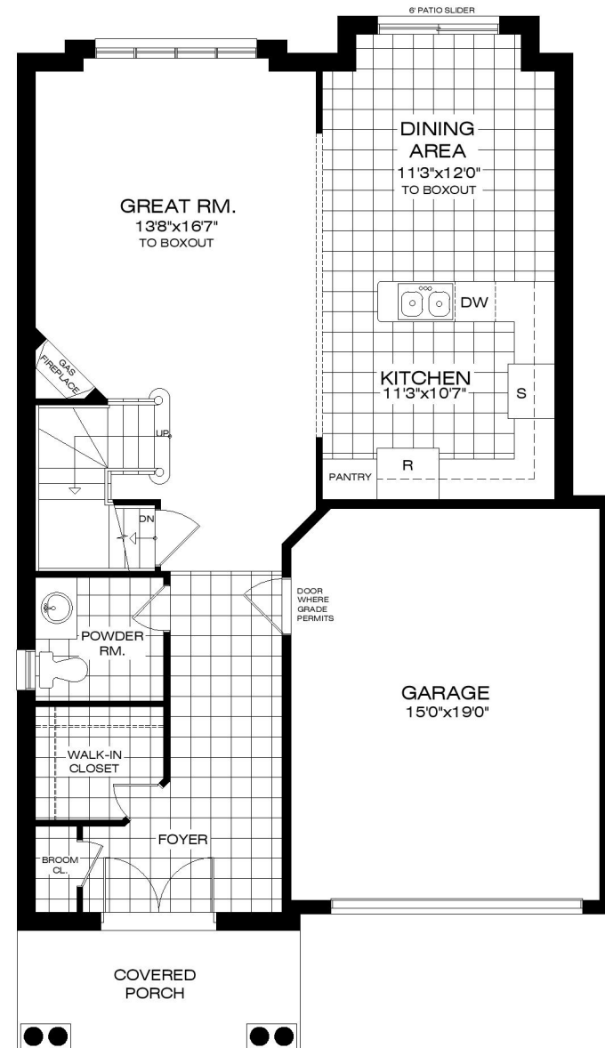
MAIN FLOOR PLAN ELEVATION A
