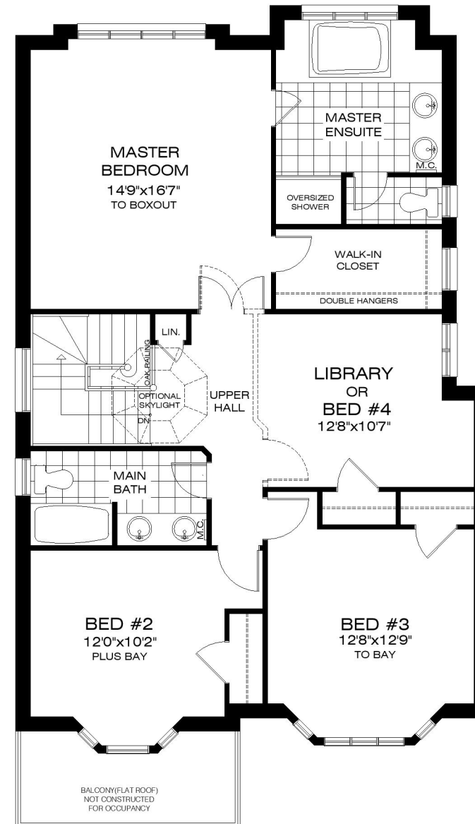
OPT. SECOND FLOOR PLAN ELEVATION A
