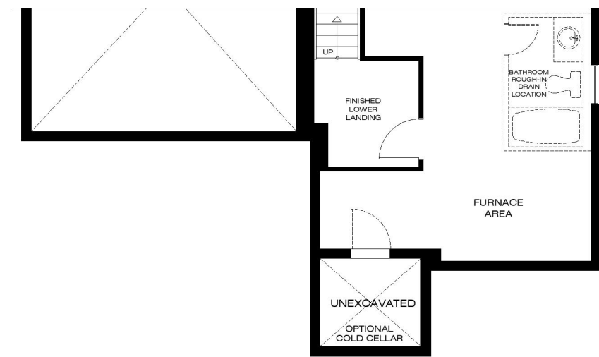
BASEMENT PLAN ELEVATION B
