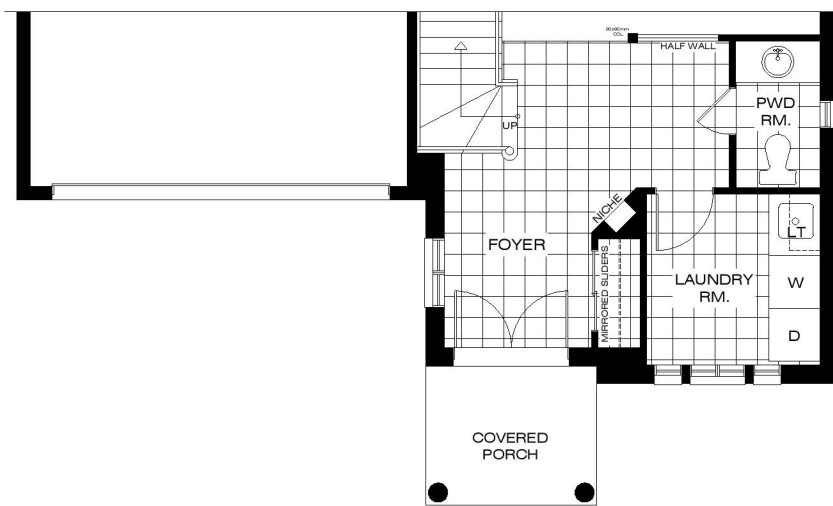
MAIN FLOOR PLAN ELEVATION B
