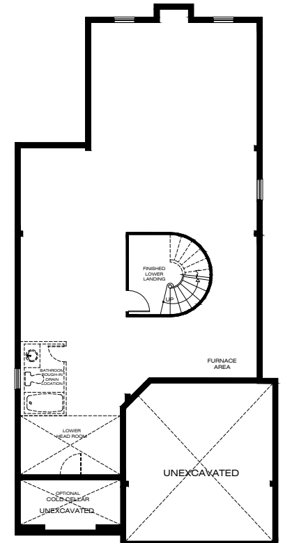
BASEMENT PLAN 'C'
