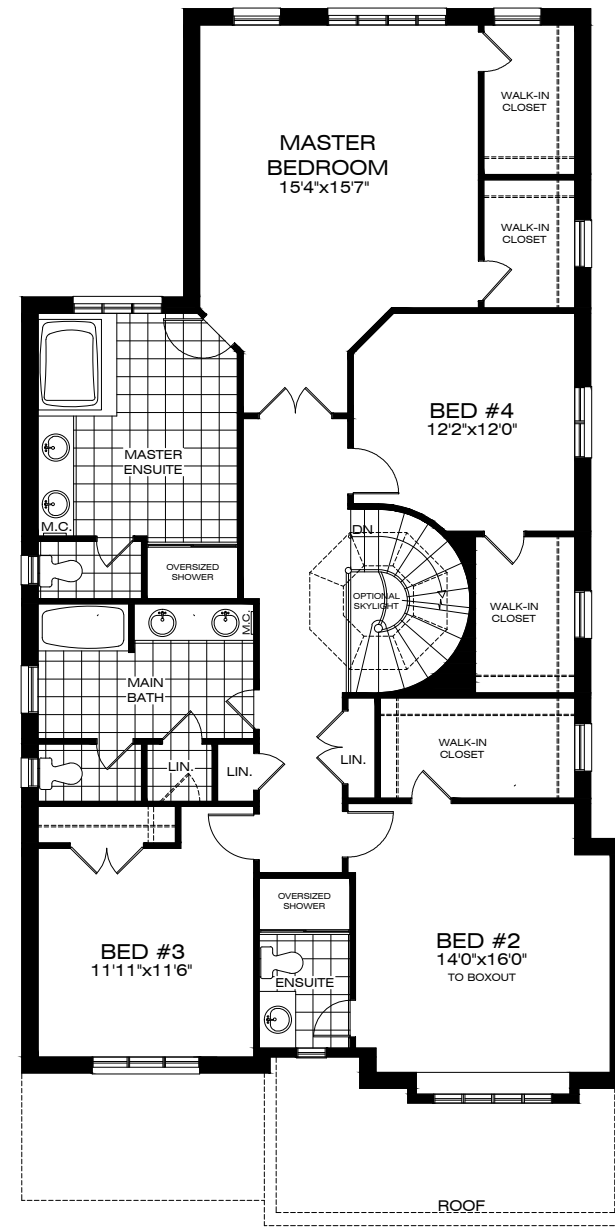
STANDARD 4 BEDROOM PLAN 'A'
