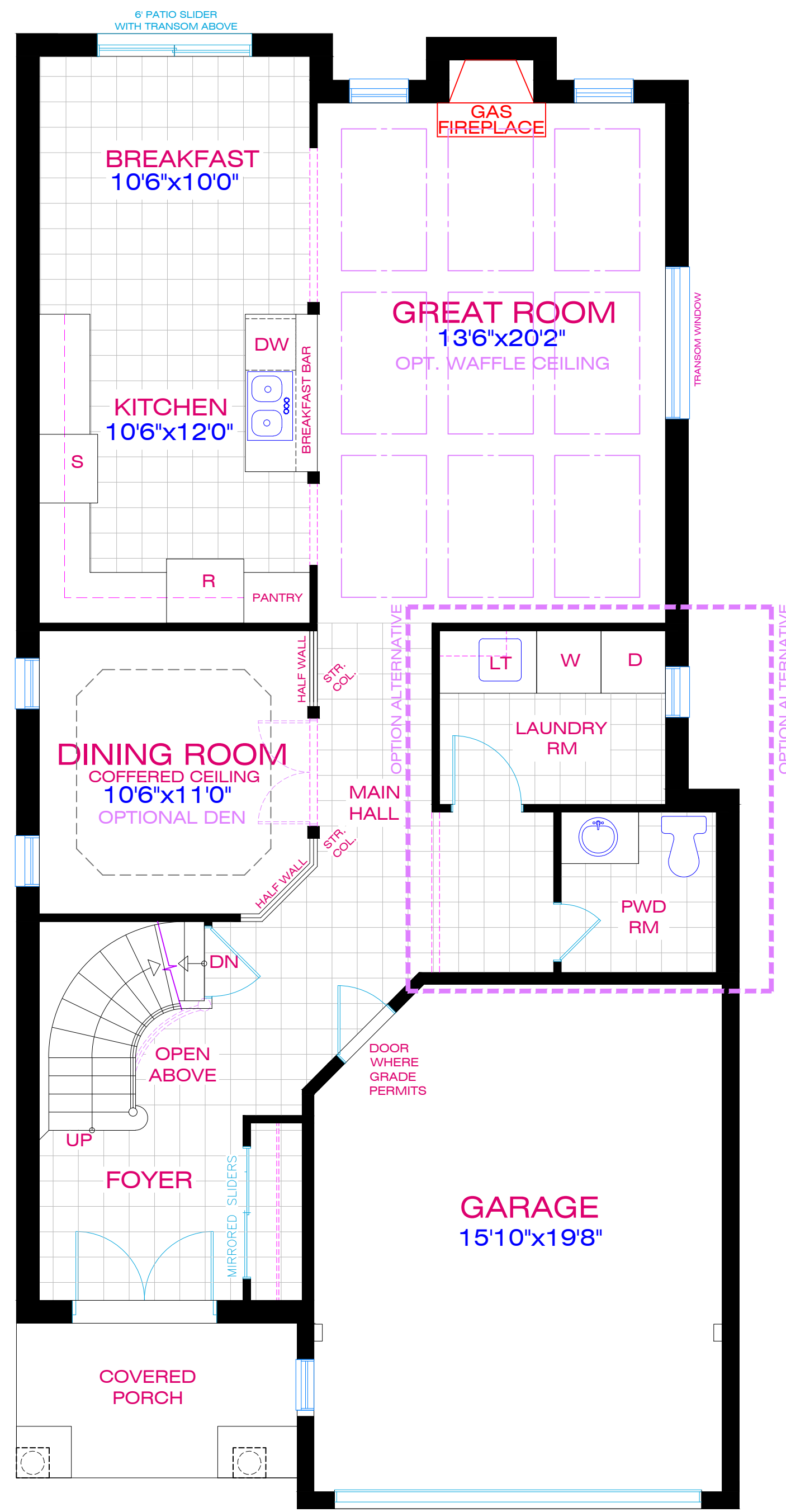
MAIN FLOOR PLAN 'A,B'
