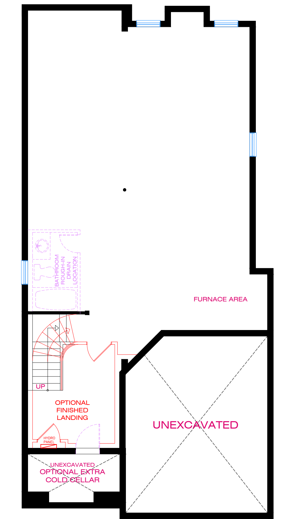
BASEMENT PLAN 'A,B' OPT. FINISHED LOWER LANDING A3-1047 The WESTBURY JOHN BODDY HOMES
