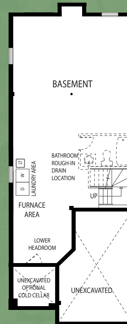
BASEMENT PLAN WITH LAUNDRY AREA END UNIT
