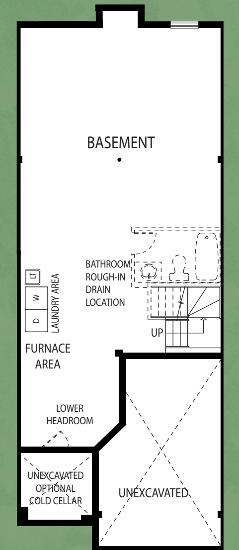
BASEMENT PLAN WITH LAUNDRY AREA INTERIOR UNIT
