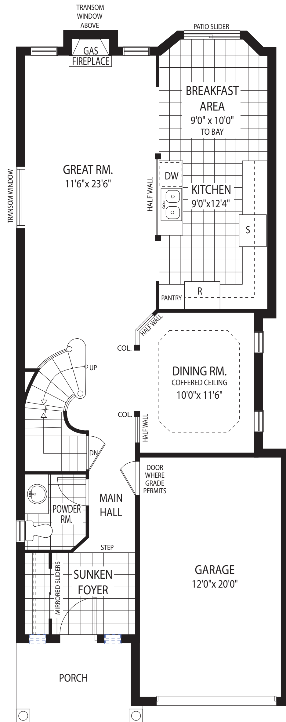
MAIN FLOOR PLAN ELEVATION A / ELEVATION B
