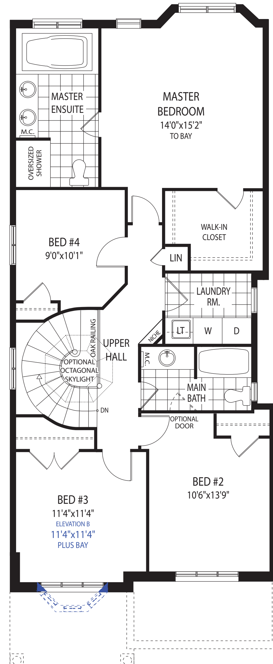
OPT. SECOND FLOOR PLAN (4 BEDROOM & LAUNDRY) ELEVATION A / ELEVATION B
