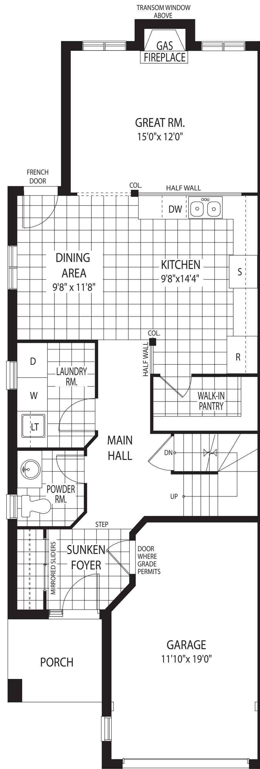
MAIN FLOOR PLAN ELEVATION A
