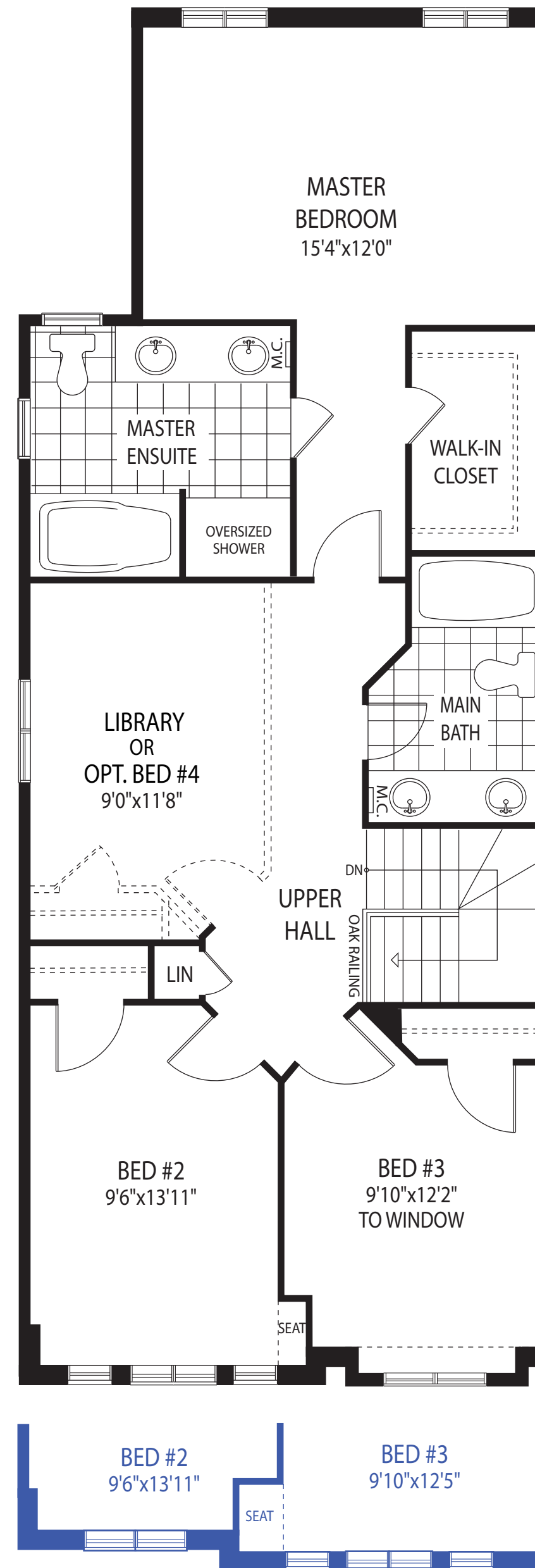
SECOND FLOOR PLAN (3 BEDROOM & LIBRARY) ELEVATION A / ELEVATION B
