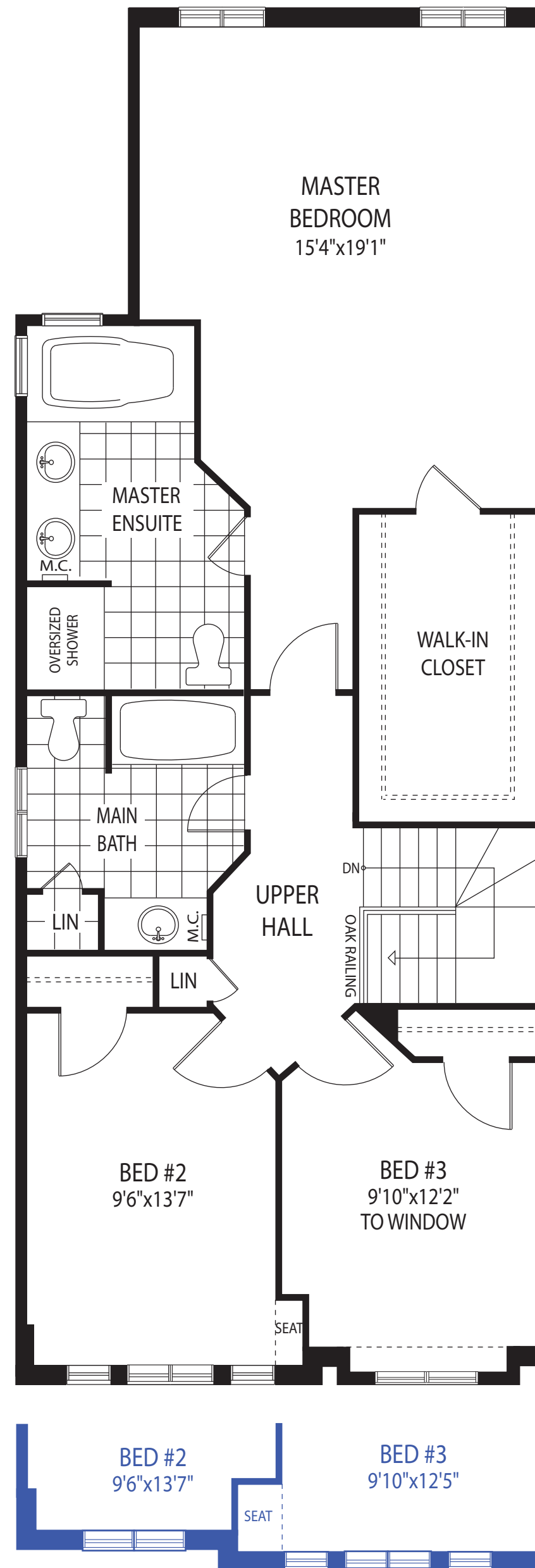
SECOND FLOOR PLAN (3 BEDROOM) ELEVATION A / ELEVATION B
