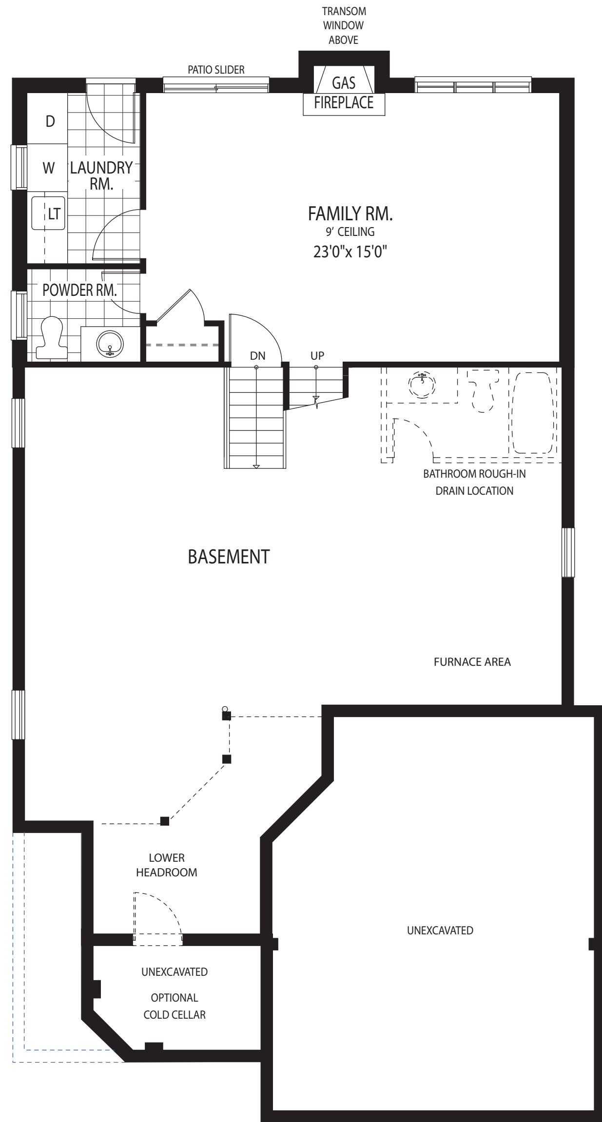
BASEMENT PLAN ELEVATION A / ELEVATION B
