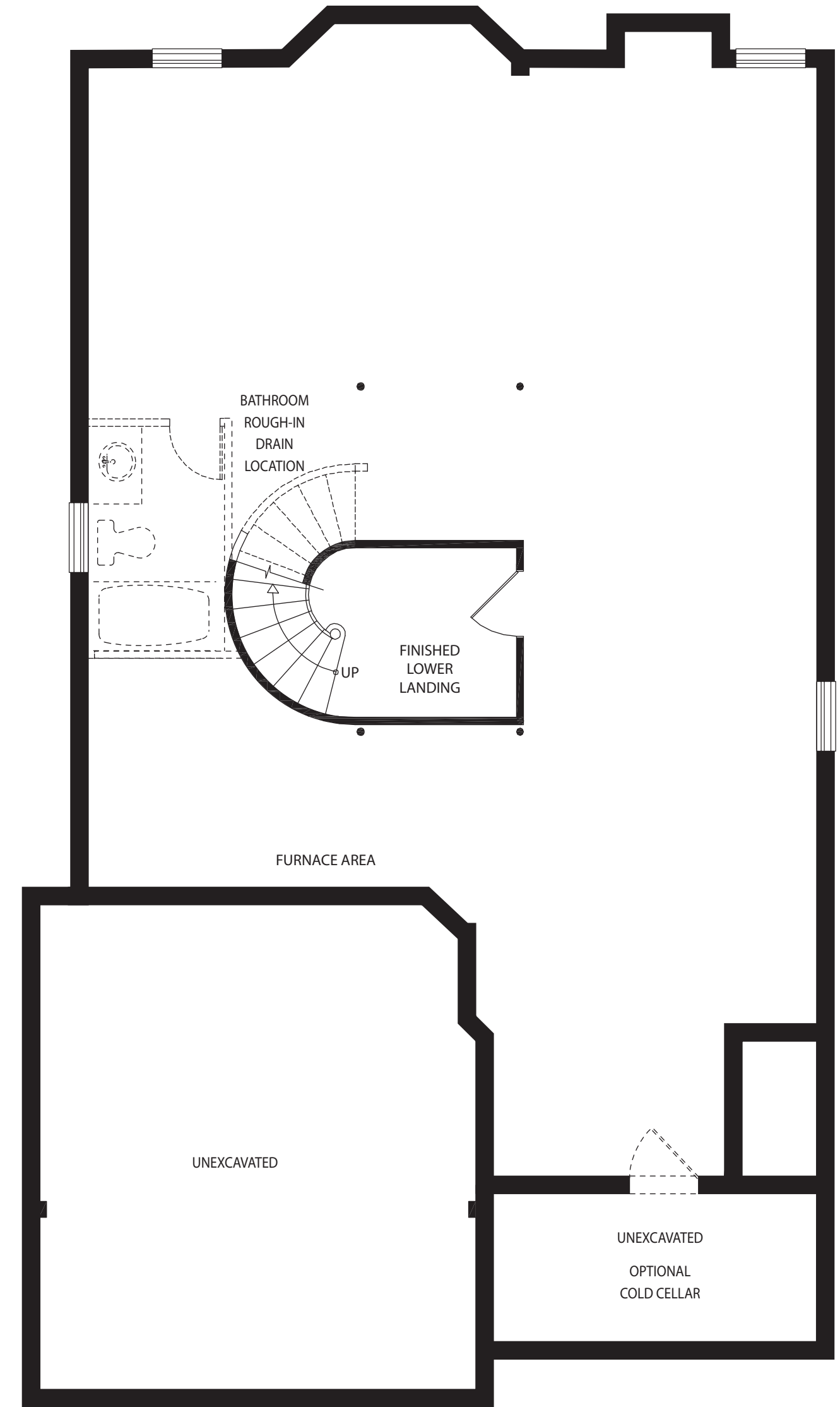
BASEMENT PLAN
