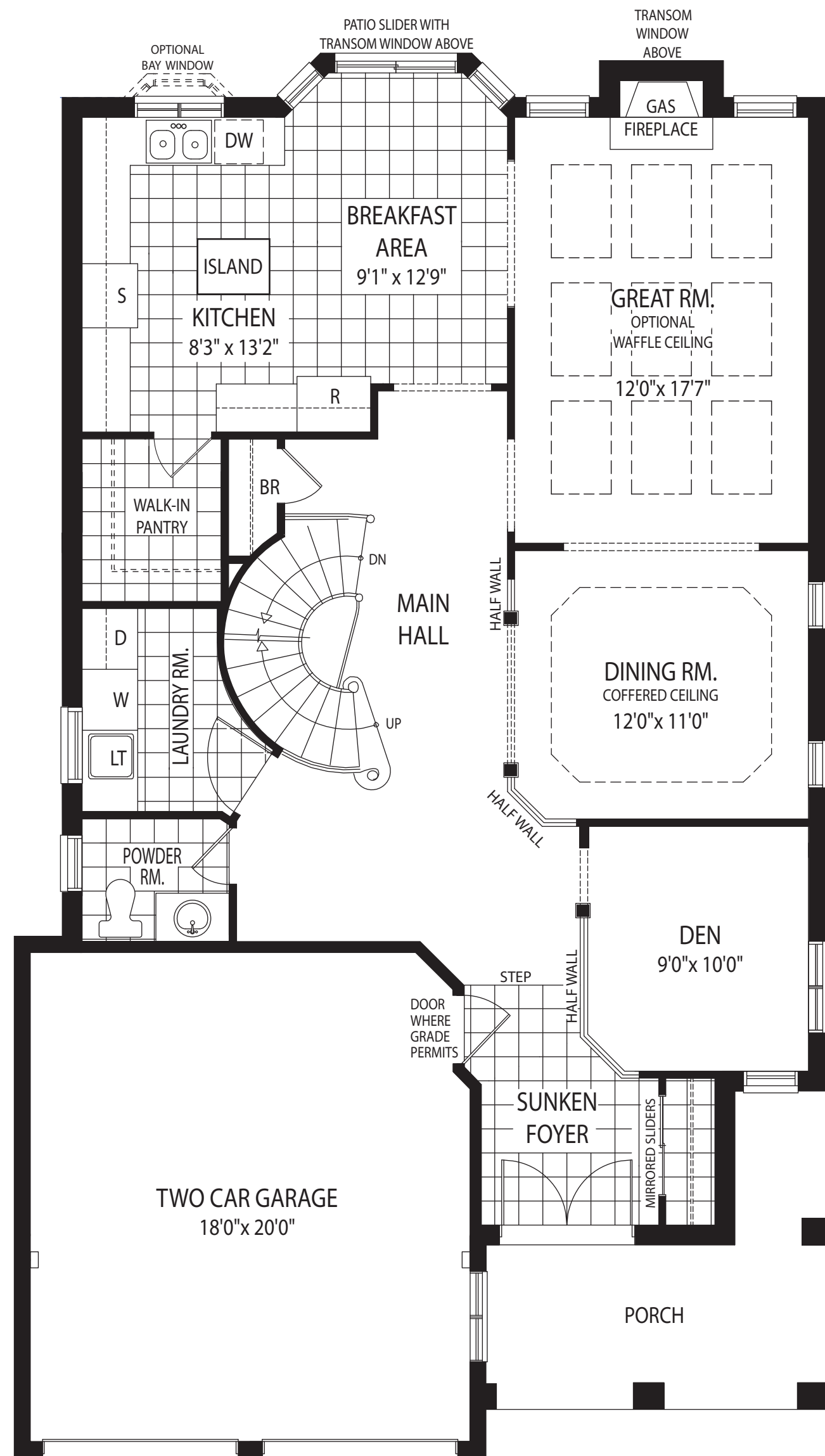
MAIN FLOOR PLAN ELEVATION A
